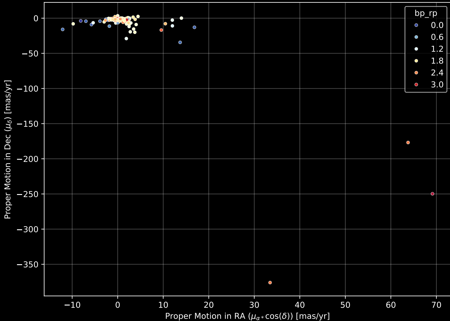
APOGEE DR17 Field: [184+04] Proper Motion Diagram (n= 186)
