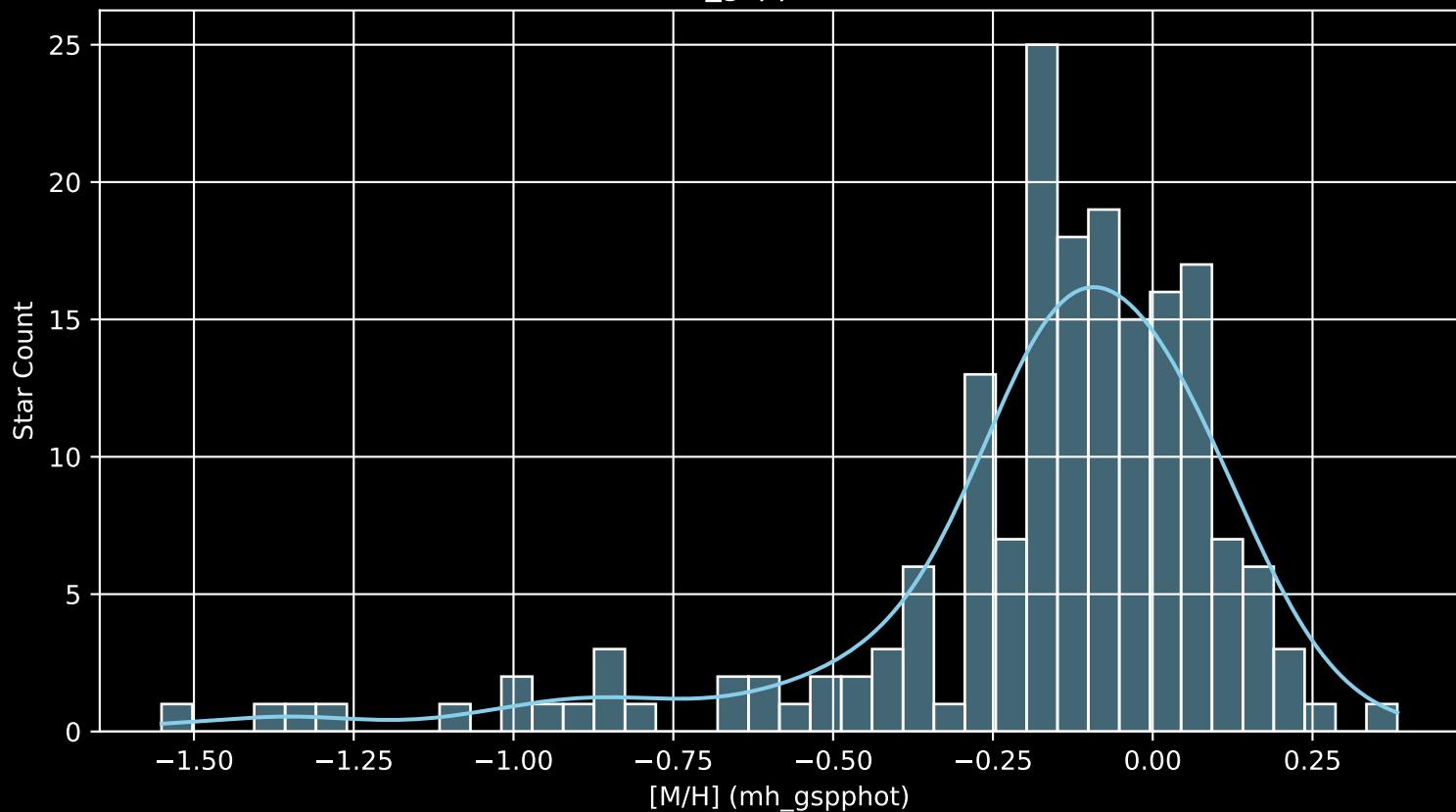
APOGEE DR17 Field: [184+04 [M/H] (mh_gspphot) (n= 180)
