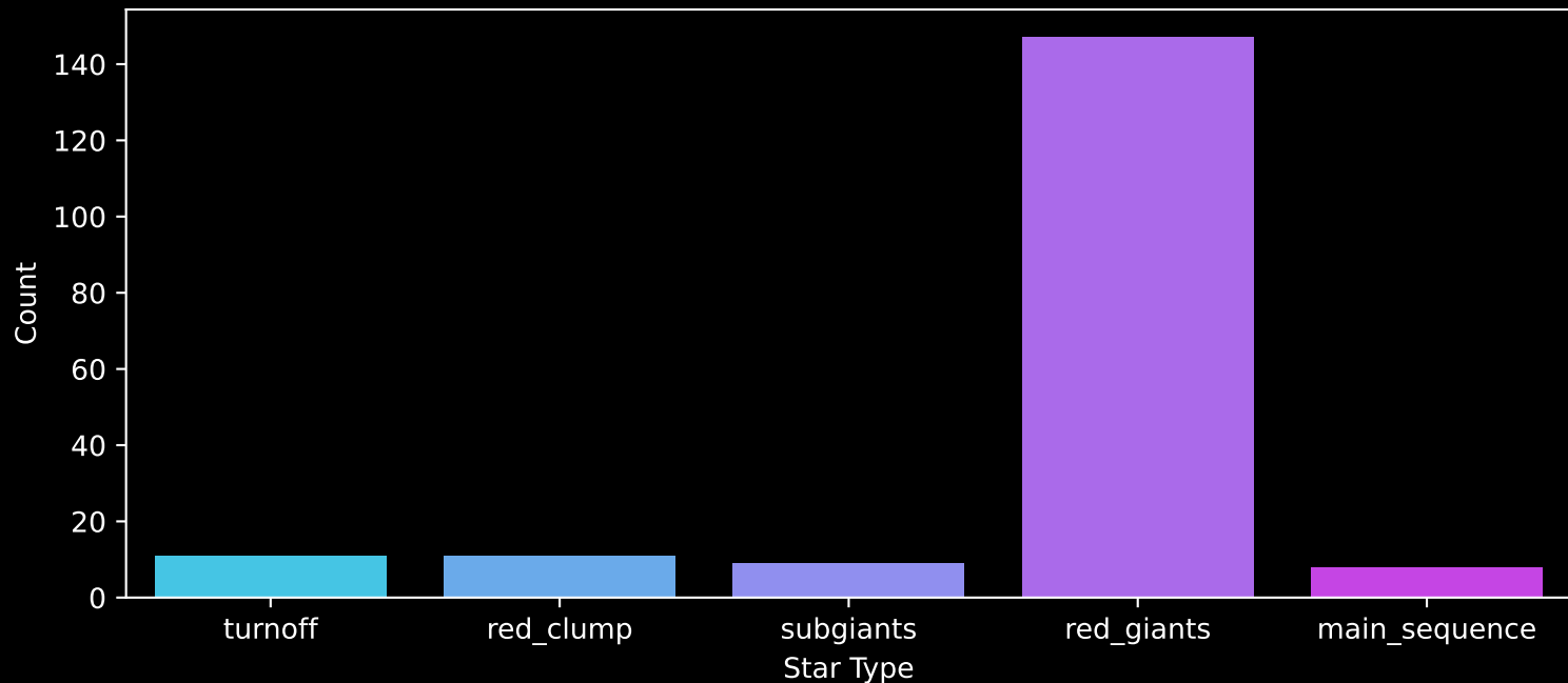
APOGEE DR17 Field: [184+04] Count plot of Star Type
