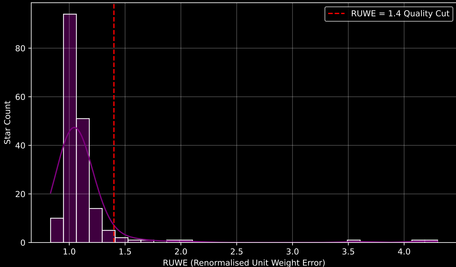
GAPOGEE DR17 Field [184+04] RUWE Distribution (n= 183)
