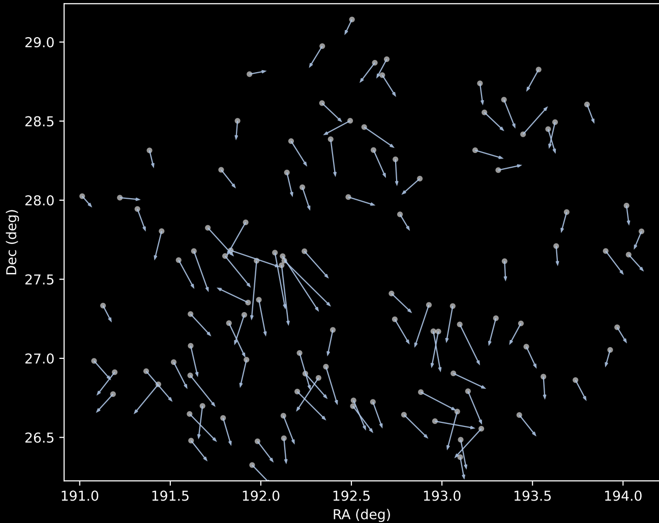
APOGEE DR17 Cluster 1 Proper Motion Vectors (n=110)
