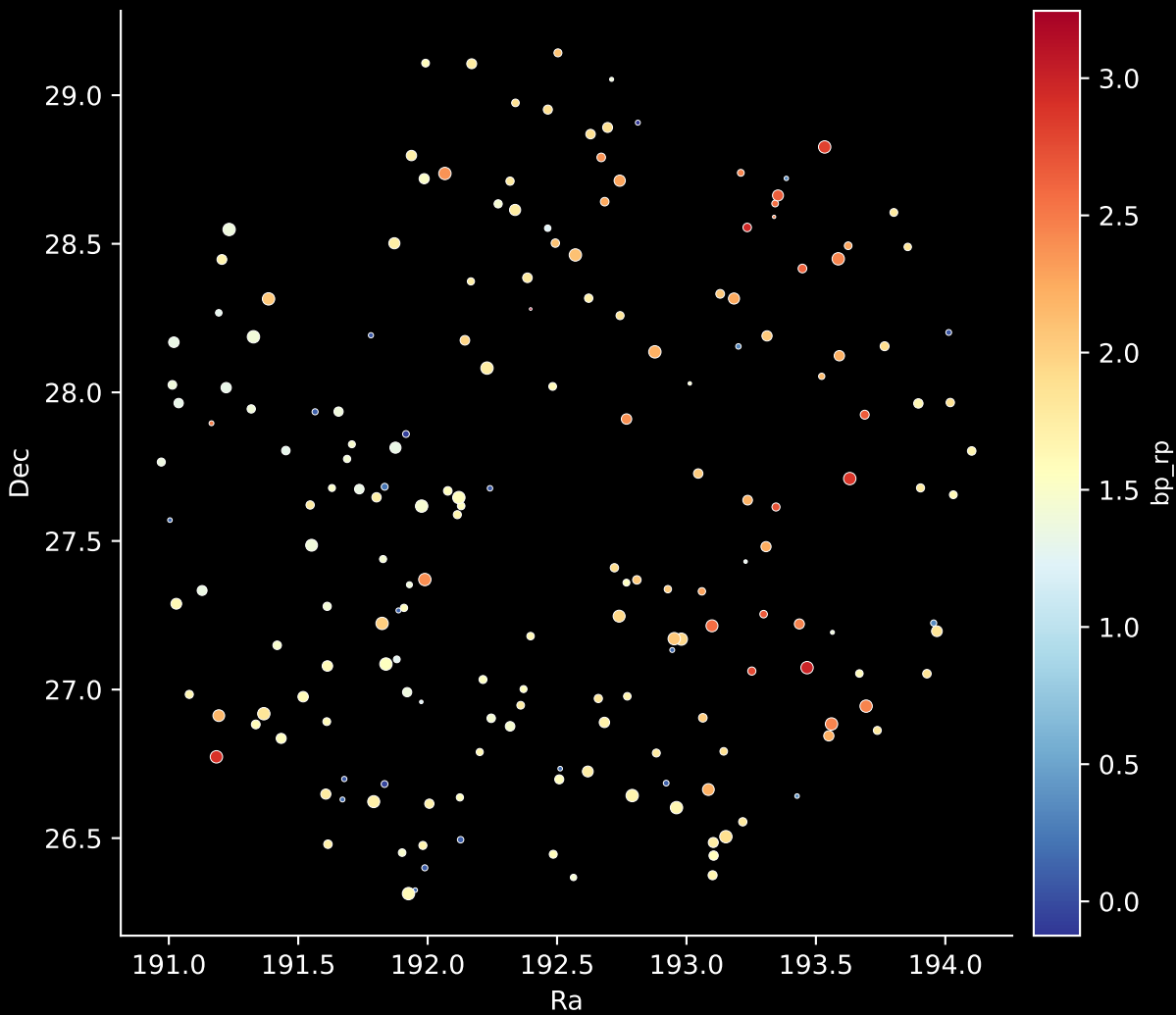
APOGEE DR17 Field: [184+04] Stars: 186
