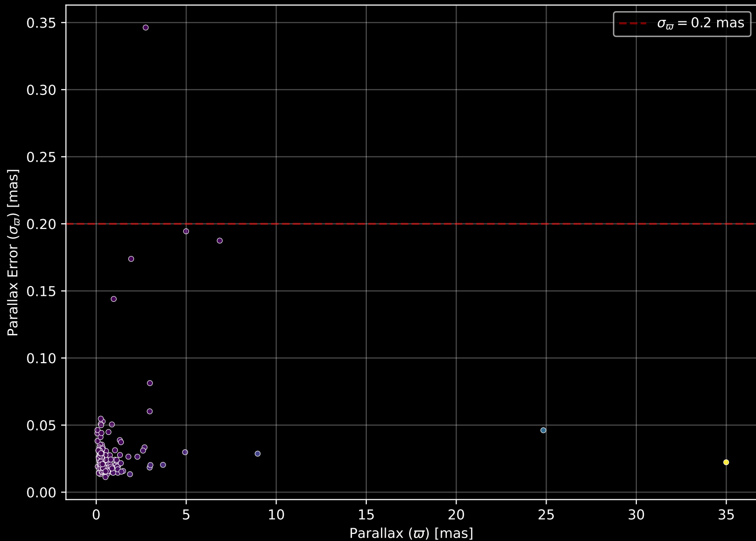
APOGEE DR17 Field: [184+04] Parallax Quality (n= 186)
